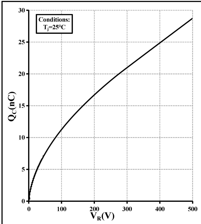
Figure 5: Total Capacitive Charge vs Reverse Voltage
