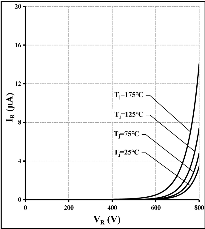
Figure 2: Reverse Characteristics
