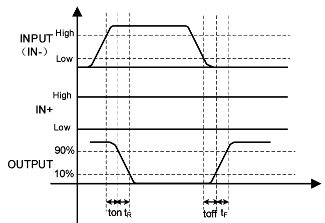
Figure 2 Input-Output waveform(inverting)
