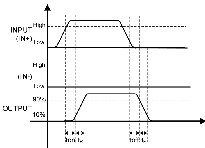
Figure 1 Input-Output waveform(non-inverting)
