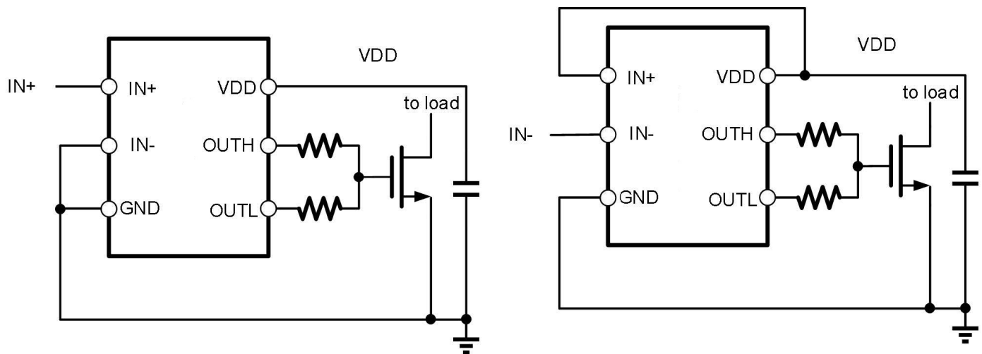
Figure 3 Typical Application Diagram of TPG27511
